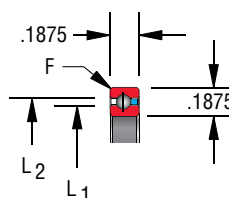
Snap-over separator 3/32" balls
