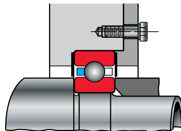
Figure 2-7 Washer Shield From Precision Flat Stock
