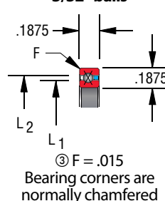
Snap-over separator 3/32" balls
