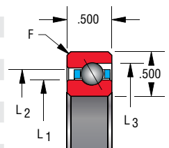
Circular pocket separator 1/4" balls
