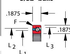
Circular pocket separator 3/32" balls
