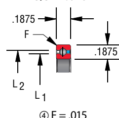
Snap-over separator 3/32" balls
