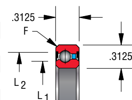
Snap-over separator 5/32" balls
