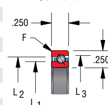
Circular pocket separator 1/8" balls
