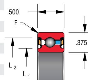
Snap-over separator 3/16" balls
