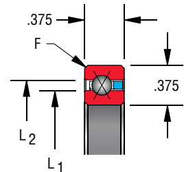
Snap-over separator 3/16" balls
