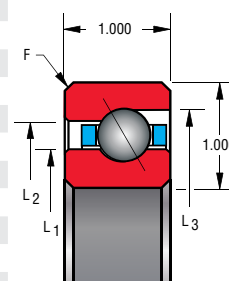
Circular pocket separator 1/2" balls
