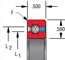
Snap-over separator 1/4" balls
