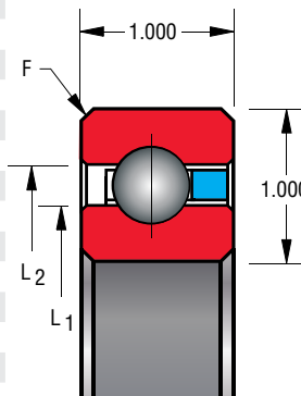
Snap-over separator 1/2" balls
