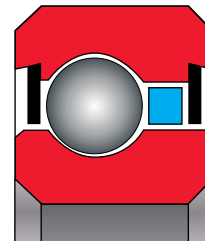
Figure 2-4 Double-Shielded Real-Slim EA/EB bearing
