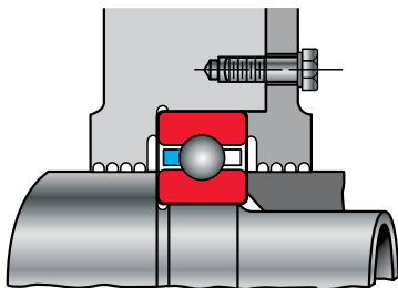
Figure 2-6 Annular Grooves
