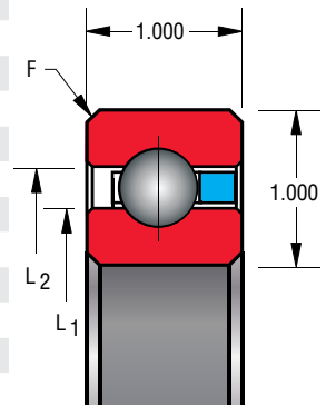
Snap-over separator 1/2" balls
