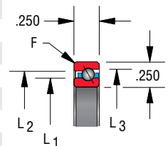
Circular pocket separator 1/8" balls
