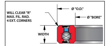
Sealed Bearing
