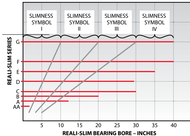
Figure 4-7 - Slimness Symbol ( S_s )
