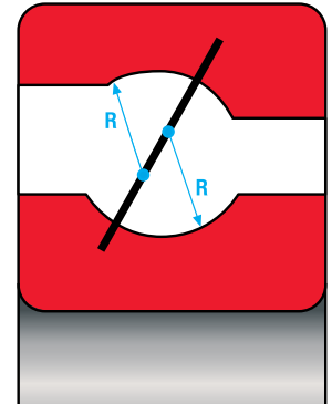
Figure 3-7 Type A
