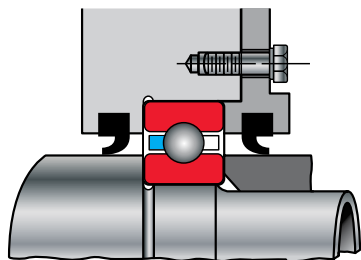
Figure 2-5 Nitrile Lip-Type Seal
