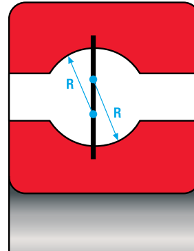
Figure 3-8 Type X
