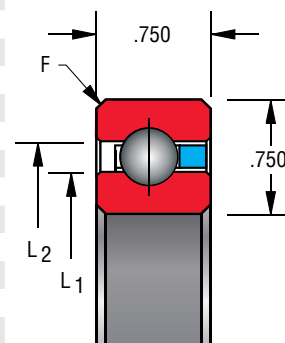
Snap-over separator 3/8" balls
