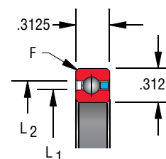
Snap-over separator 5/32" balls
