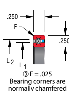
Snap-over separator 1/8" balls
