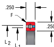
Snap-over separator 1/8" balls
