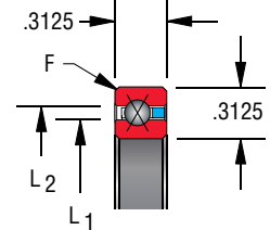
Snap-over separator 5/32" balls
