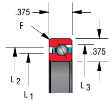
Circular pocket separator 3/16" balls
