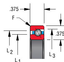
Circular pocket separator 3/16" balls
