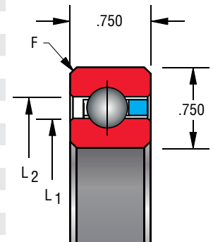
Snap-over separator 3/8" balls
