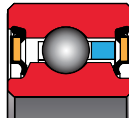
Figure 2-3 Double-Sealed Real-Slim JG bearing
