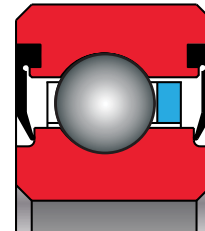
Figure 2-4 Double-Shielded Real-Slim EA/EB bearing
