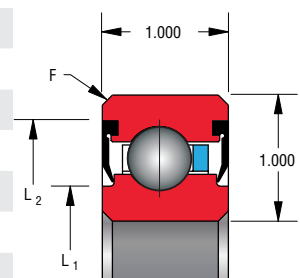
Snap-over separator 1/2" balls
