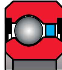
Figure 2-2 Double-Sealed Real-Slim JU bearing
